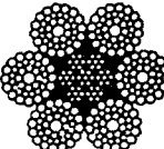
6 x 49 FILLER WIRE-SEALE
