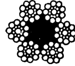
6 x 19 SEALE
