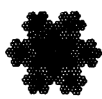
6 x 42 (TILLER ROPE)
