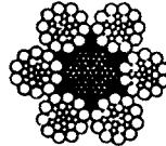
6 x 26 WARRINGTON-SEALE (LOGGING ROPE)
