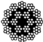
18 x 7 (NON-ROTATING ROPE)
