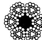
6 x 25 STYLE B FLATTENED STRAND
