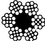
6 x 17 FILLER WIRE (HAULAGE ROPE)
