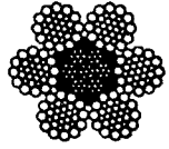
6 x 31 WARRINGTON-SEALE
