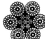
6 x 55 SEALE-WARRINGTON
