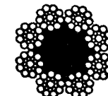
8 x 19 SEALE
