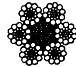
6 x 27 SEALE (LOGGING ROPE)
