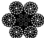
6 x 41 WARRINGTON-SEALE
