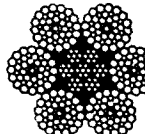
6 x 49 SEALE-WARRINGTON-SEALE
