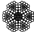
6 x 30 STYLE G FLATTENED STRAND
