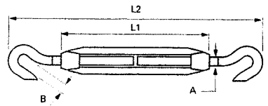
Turnbuckles Hook & Hook Stainless Steel Type 316 Forged
