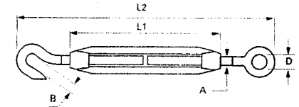
Turnbuckles Eye & Hook Stainless Steel Type 316 Forged
