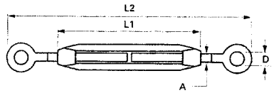
Turnbuckles Eye & Eye Stainless Steel Type 316 Forged
