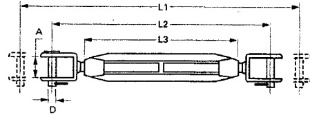
Turnbuckles Welded Forks Stainless Steel Type 316 Forged
