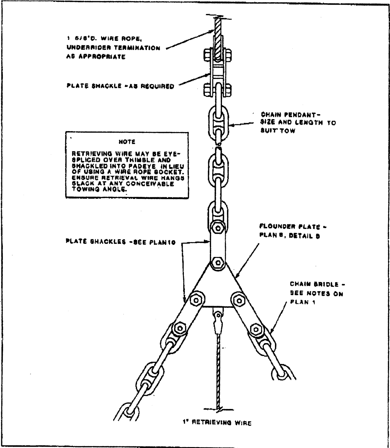
Towing Plan No. 7 - Chain Bridle and Pendant in Christmas Tree Rig.
