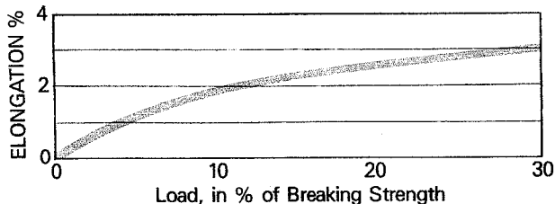
Load-Elastic Elongation Curve for Stabilized True-Blue Rope Under Cyclic Loading
